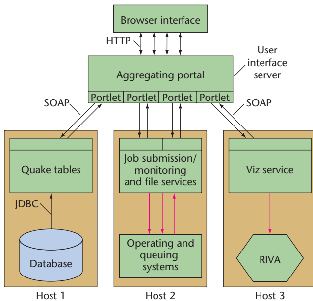
Figure 2. QuakeSim portal and service architecture. The database is the QuakeTables database; RIVA is the Remote Interactive Visualization and Analysis System. RIVA can be used as an interactive system to explore and visualize large terrain data sets in 3D perspective views, or as an animation tool to generate fly-by movies using high-resolution images and digital elevation.
