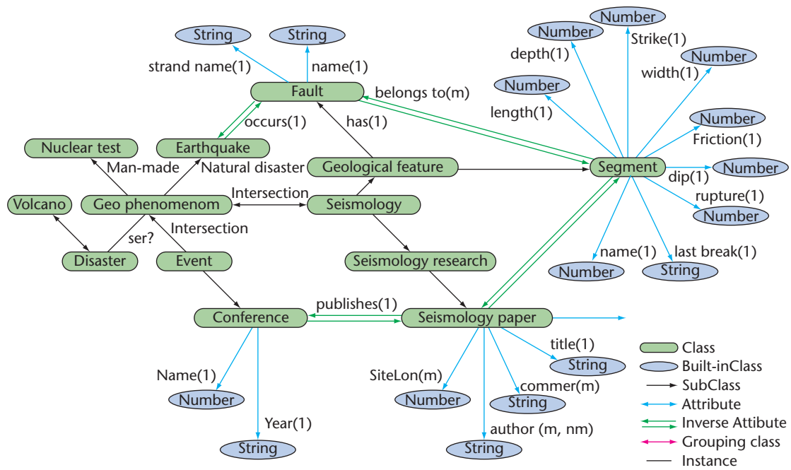
Figure 1. A seismology domain ontology (created by Ontonic). 5 The two roots in the example—event and seismology—can be further categorized. For example, seismology can be specialized as geophenomenon, seismology research, or geological feature, and event can be subcategorized as disaster, conference, or geophenomenon. Each subclass can be further specialized, as shown.
